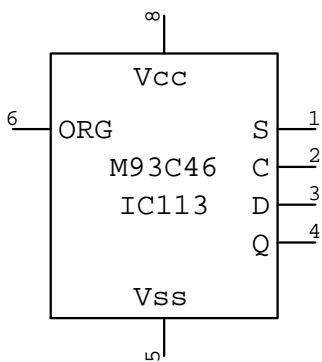
M93C46 IC???
