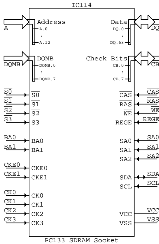
PC133SDRAM IC???
