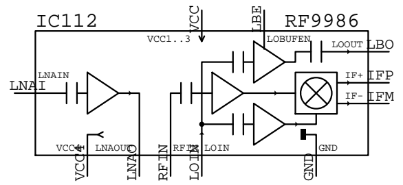
RF9986 IC???
