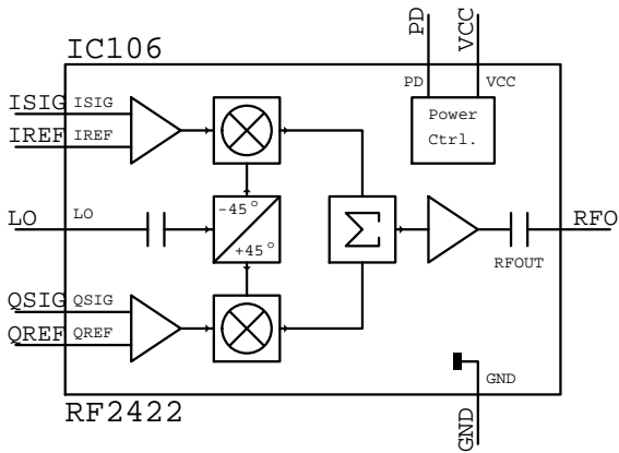
RF2422 IC???
