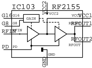
RF2155 IC???
