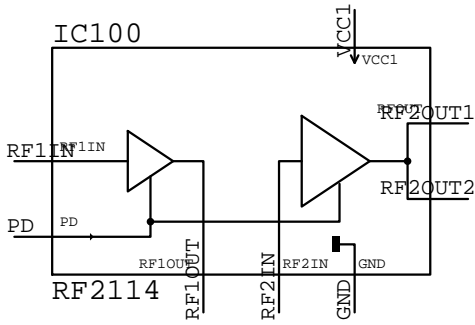
RF2114 IC???
