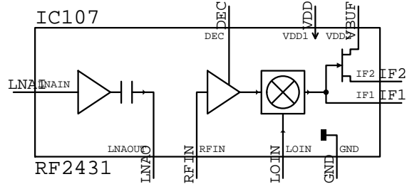
RF2431 IC???
