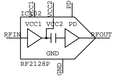
RF2128P IC???
